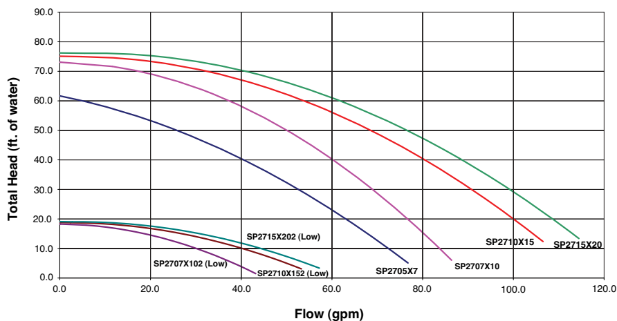
Max-Flo II Flow vs Total Head
